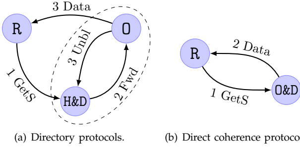
Fig. 3. How cache-to-cache transfer misses are performed in directory and direct coherence protocols. R=Requester; H=Home; D=Directory; O=Owner.
