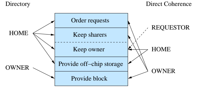
Fig. 4. Tasks performed in cache coherence protocols.
