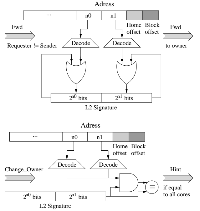
Fig. 8. Organization of the address signature mechanism proposed to send hints.
