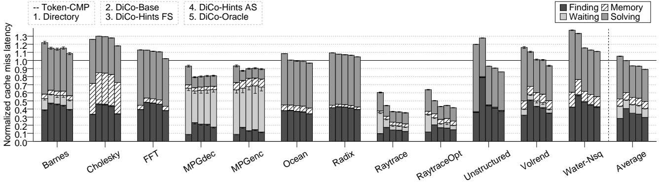
Fig. 10. Normalized L1 cache miss latency for the applications evaluated in this work.
