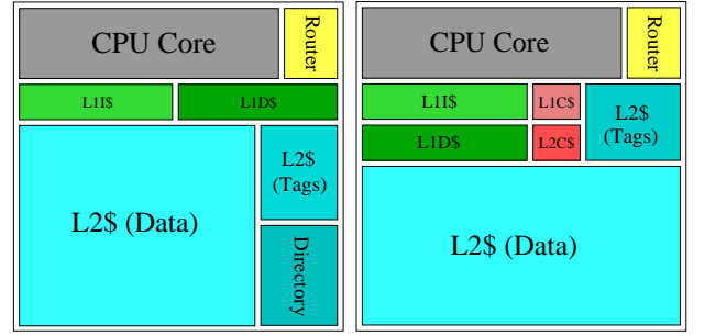
Fig. 6. Organization of a tile for a directory protocol (left) and for direct coherence (right).
