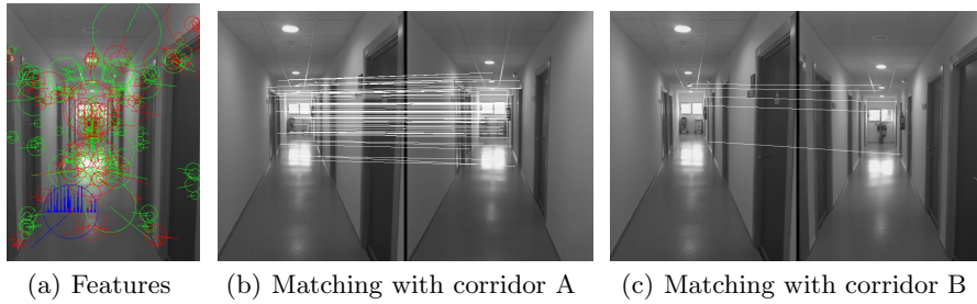
Fig. 5. SIFT features and matching of images
