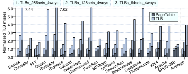
Figure 3: Distribution of TLB misses resolved by other TLBs or by the page table
