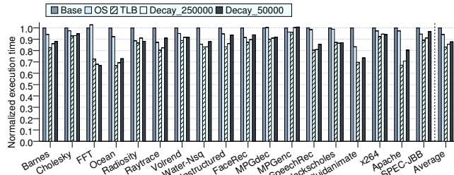
Figure 12: Execution time for coherence deactivation
