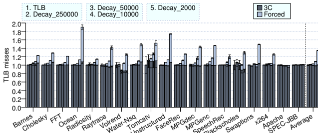
Figure 7: TLB misses
