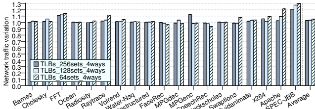
Figure 6: Network traffic using TLB-to-TLB transfers
