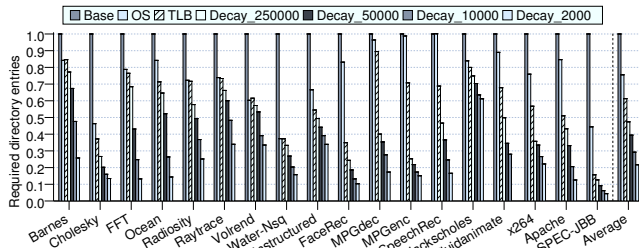
Figure 11: Average directory entries required (per cycle)
