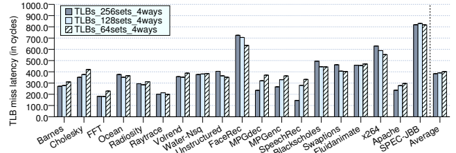
Figure 4: Average TLB miss latency
