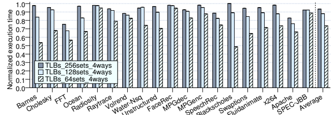
Figure 5: Execution time using TLB-to-TLB transfers
