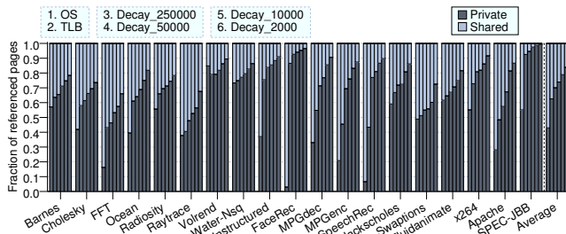
Figure 10: Private vs. shared pages
