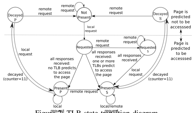
Figure 2: TLB state transition diagram.
