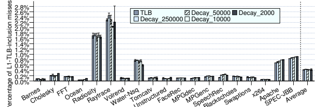
Figure 8: Percentage of L1 cache misses due to our TLB-L1 inclusion policy
