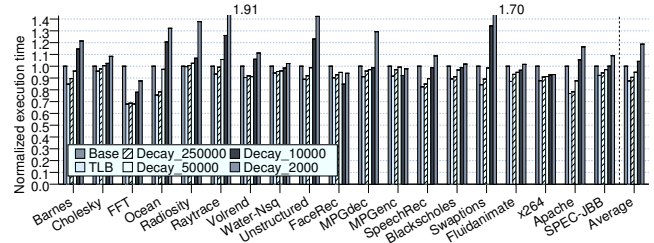
Figure 9: Execution time degradation of the decay technique
