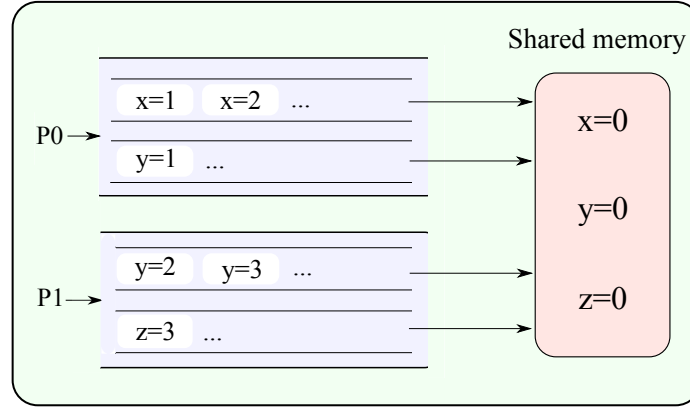
FIGURE 17. PSO
