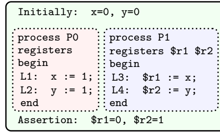
FIGURE 15. Program MP.
