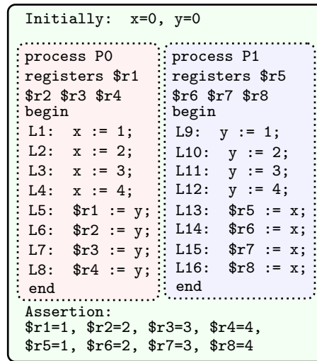
FIGURE 16. Program ReadSeq.
