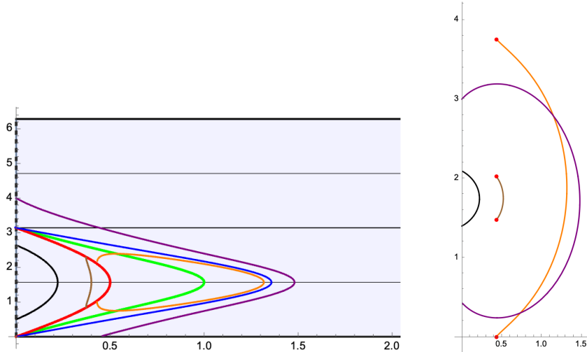
Fig. 7: Left: the orbits corresponding to the rotational \Phi -surfaces of type 1.5 – 1.8 of Th. 3.2. Right: the profile curve of the \Phi -surface corresponding to each orbit.
