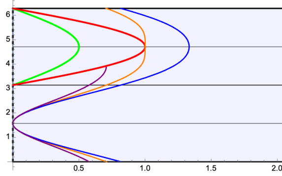
Fig. 9: The phase plane for the case b = 1 , \Phi = c \in \mathbb{R} , c < -a^2 , and the distinct orbits depending on the sign of c + 2a^2 .
