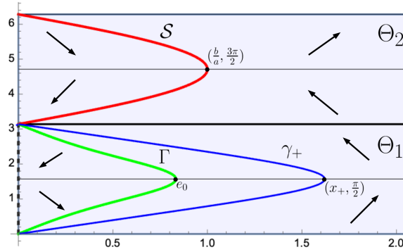
Fig. 1: The phase plane for the case a > 0, b > 0 and the orbit of the rotational sphere in blue.
