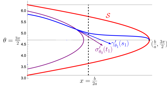
Fig. 4: The diagram of the contradiction in the proof of Claim 1.
