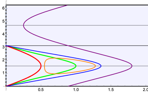
Fig. 6: The structure of the phase plane in the elliptic case for a > 0, b < 0 , and the orbits corresponding to the complete rotational \Phi -surfaces.
