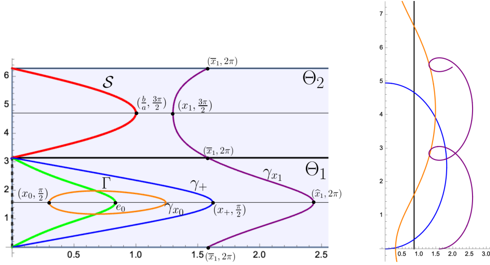
Fig. 2: Left: the phase plane for a > 0, b > 0 and a prescribed function \Phi under the hypotheses of Th. 3.1. The orbits correspond to the complete examples. Right: the profile curve of the \Phi -surface corresponding to each orbit.
