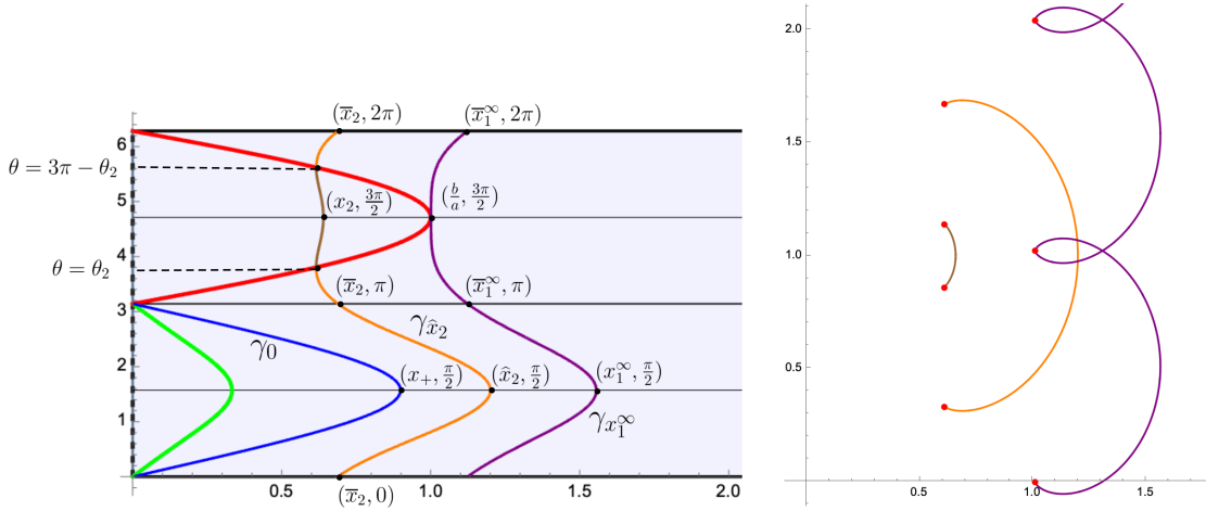
Fig. 5: Left: the orbits corresponding to the rotational \Phi -surfaces of type 1.7, 1.8 of Th. 3.1. Right: the profile curve of the \Phi -surface corresponding to each orbit.
