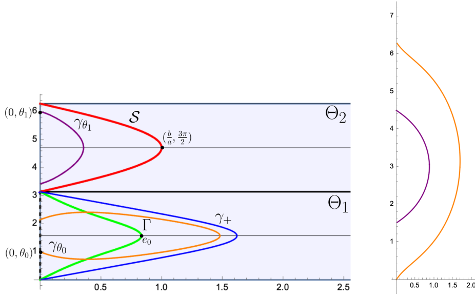
Fig. 3: Left: the orbits corresponding to the rotational \Phi -surfaces of type 1.5, 1.6 of Th. 3.1. Right: the profile curve of the \Phi -surface corresponding to each orbit.
