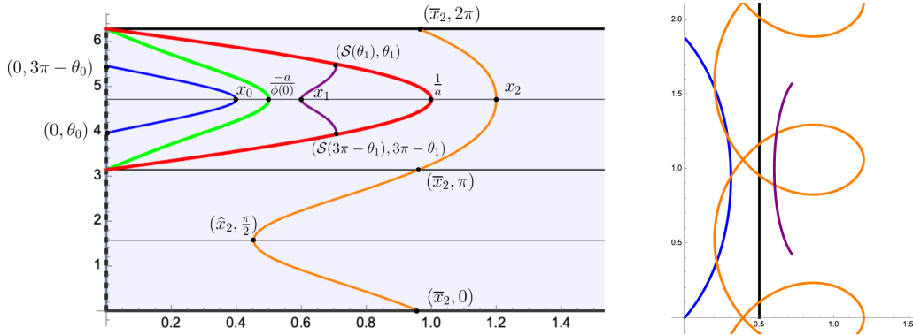
Fig. 8: Left: The phase plane for b = 1 and \Phi < -a^2 , and the orbits appearing in the statement of Th. 4.1. Right: the profile curve corresponding to such orbits.
