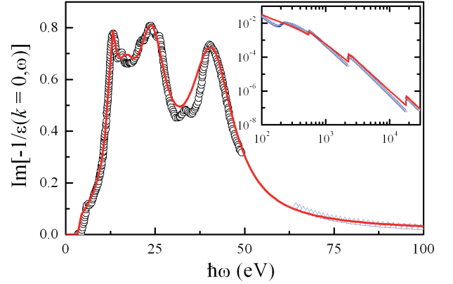
Fig. 2. (Color online) Energy loss function of ZrO 2 as a function of the transferred energy, \hbar\omega , in the optical limit ( k = 0 ). The circles correspond to experimental data from Frandon et al. [29], the solid line represents the ELF obtained through the MELF-GOS model [18,19] and the triangles (at \hbar\omega \geq 60 eV) are data derived from X-ray scattering factors from Henke et al. [32].
