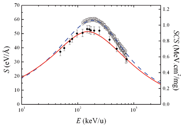
Fig. 4. (Color online) Stopping power (left axis) of a \text{ZrO}_2 film for an \alpha -particle beam as a function of the incident energy. The full circles stand for the experimental results obtained in this work, open squares correspond to previous experiments with an error of 4% [13], the full line represents our theoretical calculation using the MELF-GOS model and the dashed line is the prediction of the SRIM-2008 code [34,35]. The right axis represents the stopping cross section.
