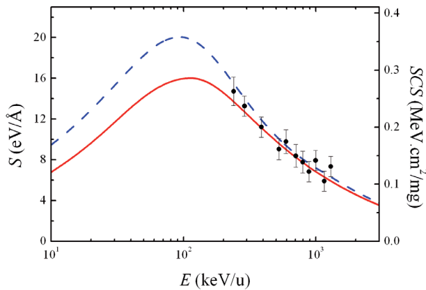
Fig. 3. (Color online) Stopping power (left axis) of a \text{ZrO}_2 film for a proton beam as a function of the incident energy. The symbols represent the experimental results, the full line represents our theoretical calculation using the MELF-GOS model and the dashed line is the prediction of the SRIM-2008 code [34,35]. The right axis represents the stopping cross section.
