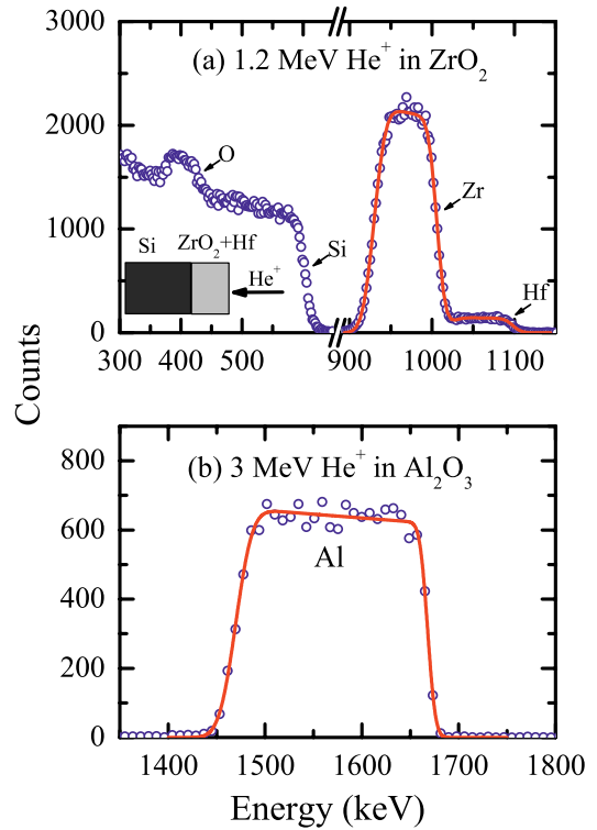
Fig. 1. (Color online) (a) Rutherford backscattering spectrum corresponding to a 1.2 MeV alpha-particle beam incident on a 95 nm-thick ZrO 2 film with an angle of incidence 30°. (b) Detail of the Al signal corresponding to the Rutherford backscattering spectrum of a 3 MeV alpha-particle beam incident at an angle 30° on a 150 nm-thick Al 2 O 3 film. The line denotes the fitting to the experimental results (symbols), which was used to extract the energy-loss straggling. The Si(Li) particle detector is located at 170° with respect to the incident beam direction.
