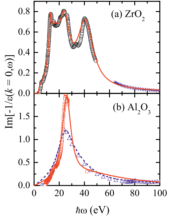
Fig. 2. (Color online) (a) Optical energy-loss function of ZrO 2 ; symbols correspond to experimental values from [32] (o) and from [33] (+) in two different regions, whereas line represents the fitting from the MELF-GOS model. (b) Optical energy-loss function of Al 2 O 3 with symbols representing two different sets of experimental data covering the same region: \Delta [34] and \square [35]. Lines represent the corresponding fitting curves obtained by the MELF-GOS model.
