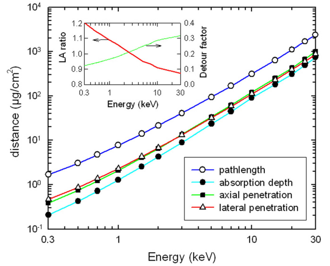
FIG. 2. (Color online) Monte Carlo simulations of the density-normalized pathlength ( \rho\bar{r}_{total} ), absorption depth ( \rho\bar{z}_n ), axial penetration ( \rho\bar{z}_{max} ), and lateral penetration ( \rho\bar{p}_{max} ) of an electron beam in MWCNT materials as a function of beam energy. The inset depicts the lateral-to-axial (LA) penetration ratio ( \frac{\rho\bar{p}_{max}}{\rho\bar{z}_{max}} ) and the detour factor ( \frac{\rho\bar{z}_n}{\rho\bar{r}_{total}} ). The lines are to guide the eye.
