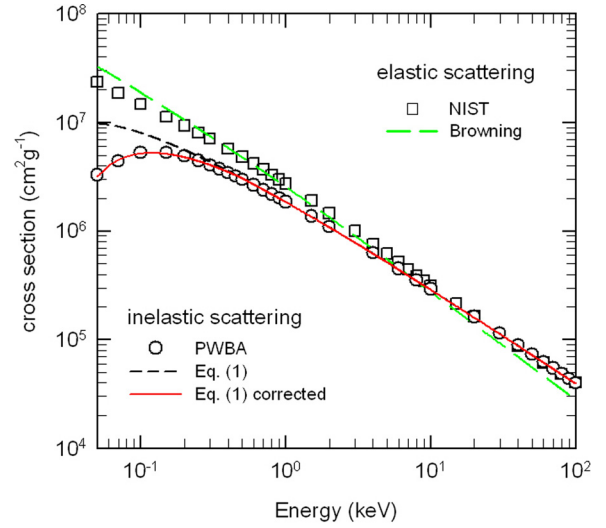
FIG. 1. (Color online) Cross section (per unit mass) for elastic and inelastic electron scattering in MWCNT materials as a function of electron energy. The PWBA and NIST results for comparison are from Refs. 33 and 35, respectively.
