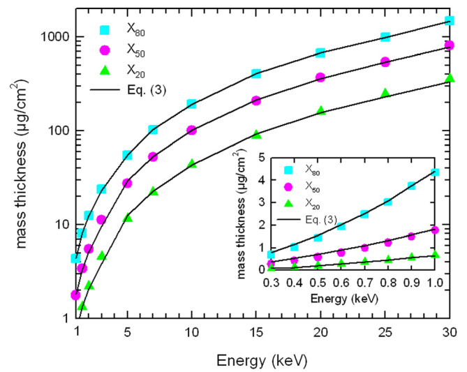
FIG. 3. (Color online) Mass thickness ( \rho z ) of MWCNT material where 20% ( X_{20} ), 50% ( X_{50} ), and 80% ( X_{80} ) of the beam energy is dissipated for electron-beam energies of 1–30 keV (main panel) and 0.3–1 keV (inset). Symbols are Monte Carlo simulations whereas the lines are analytical calculations using Eq. (3).
